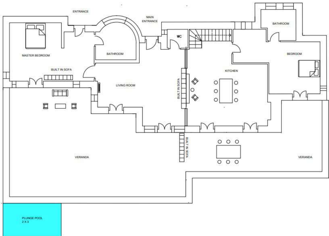
VILLA 4 GROUND FLOOR 180 sqm
